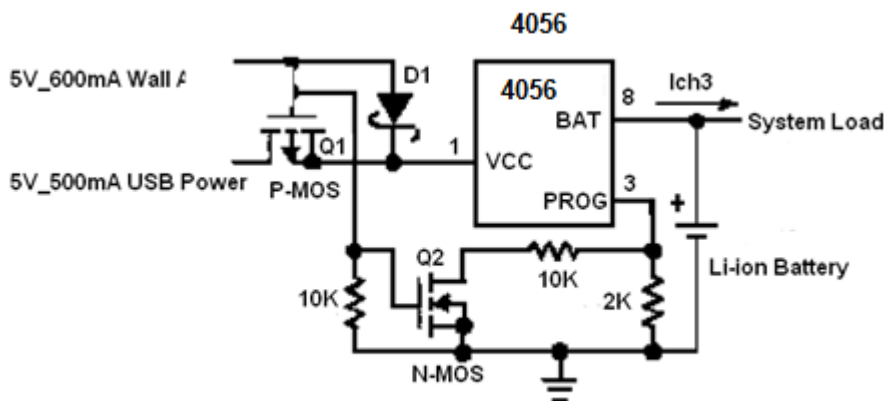
Fig.5:Combining Wall Adapter and USB Power
