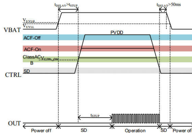
Fig. 7 Pop-Click Noise Reduction by Shutdown
