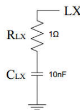
Fig. 2 LX Terminal Configuration
