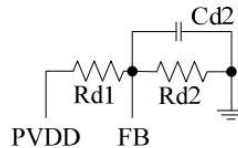
Fig. 1 FB Terminal Configuration
