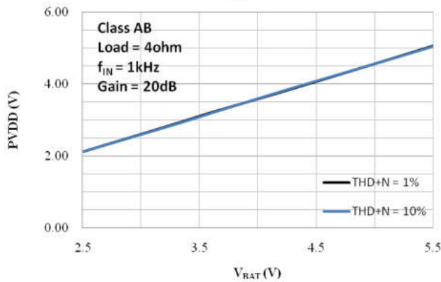
V_{BAT} vs P_{VDD}
