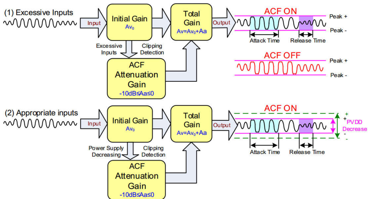
Fig. 6 the ACF Function Operation Outline
