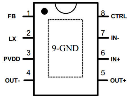
SOP8L-PP Top View
